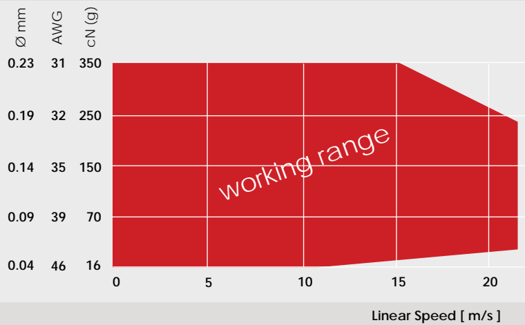
Wire / Tension
